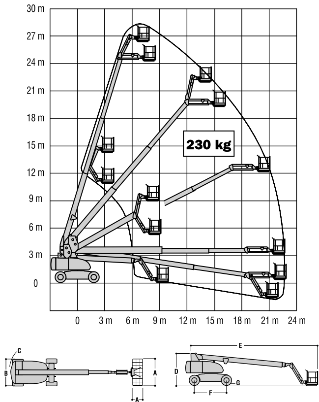
860SJ JLG modell
